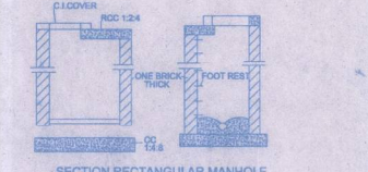
SECTION RECTANGULAR MANHOLE
