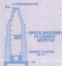
SECT. DETAILS OF FOOT REST
