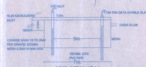
SECT. DETAIL AT 1-1
