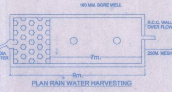
PLAN RAIN WATER HARVESTING
