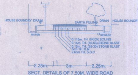
SECT. DETAILS OF 7.50M. WIDE ROAD
