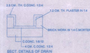
SECT. DETAILS OF DRAIN
