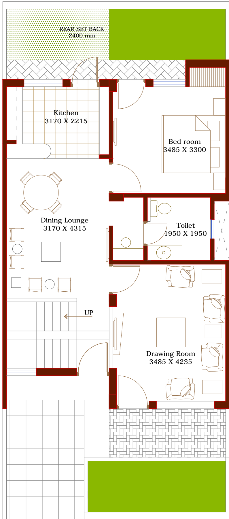
GROUND FLOOR PLAN VILLA
