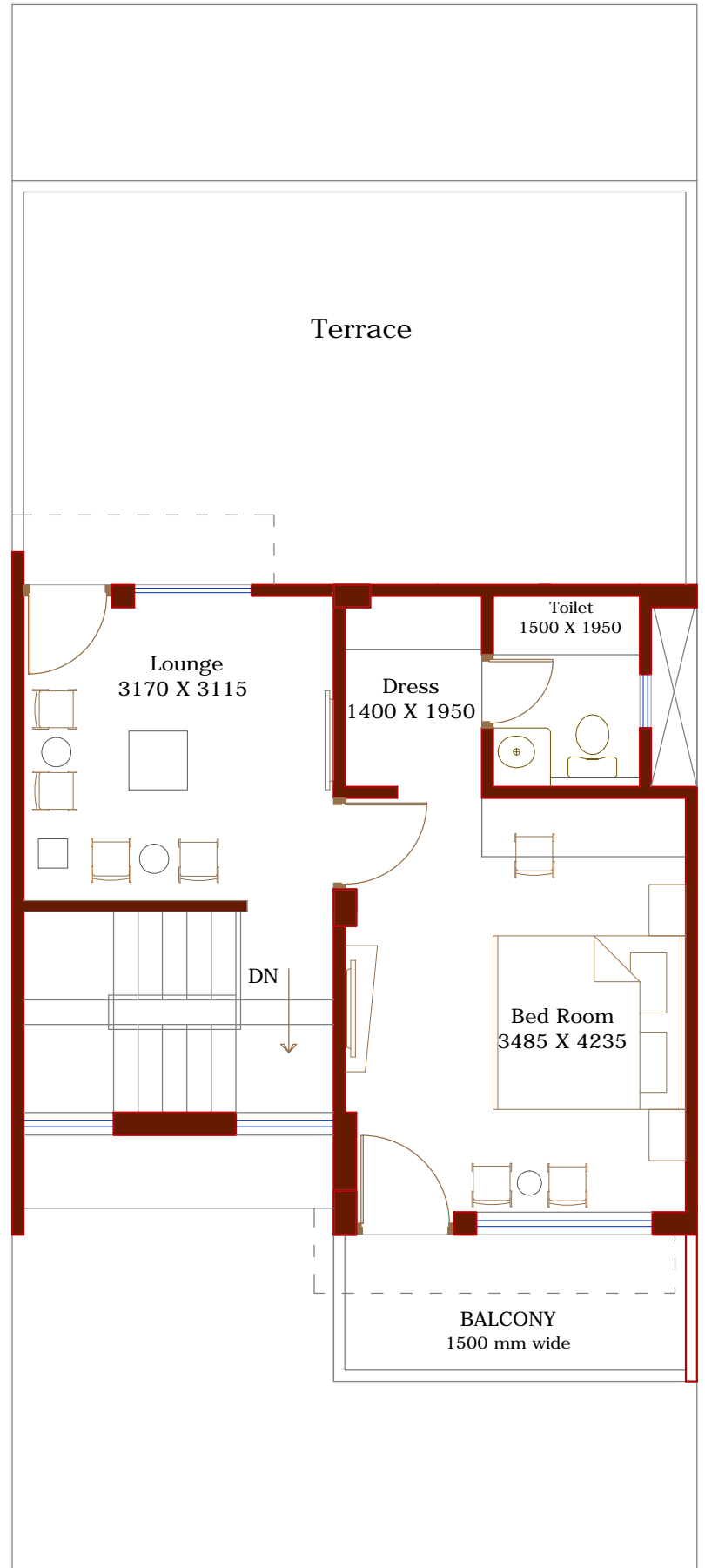
FIRST FLOOR PLAN VILLA
