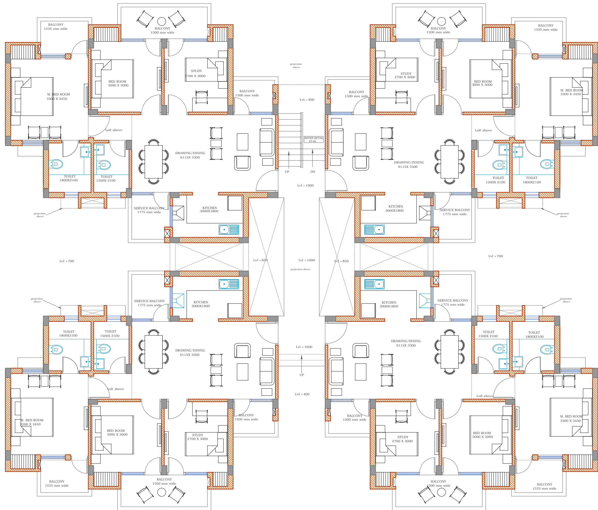
GROUND FLOOR PLAN 2+ STUDY BED ROOM APARTMENT
