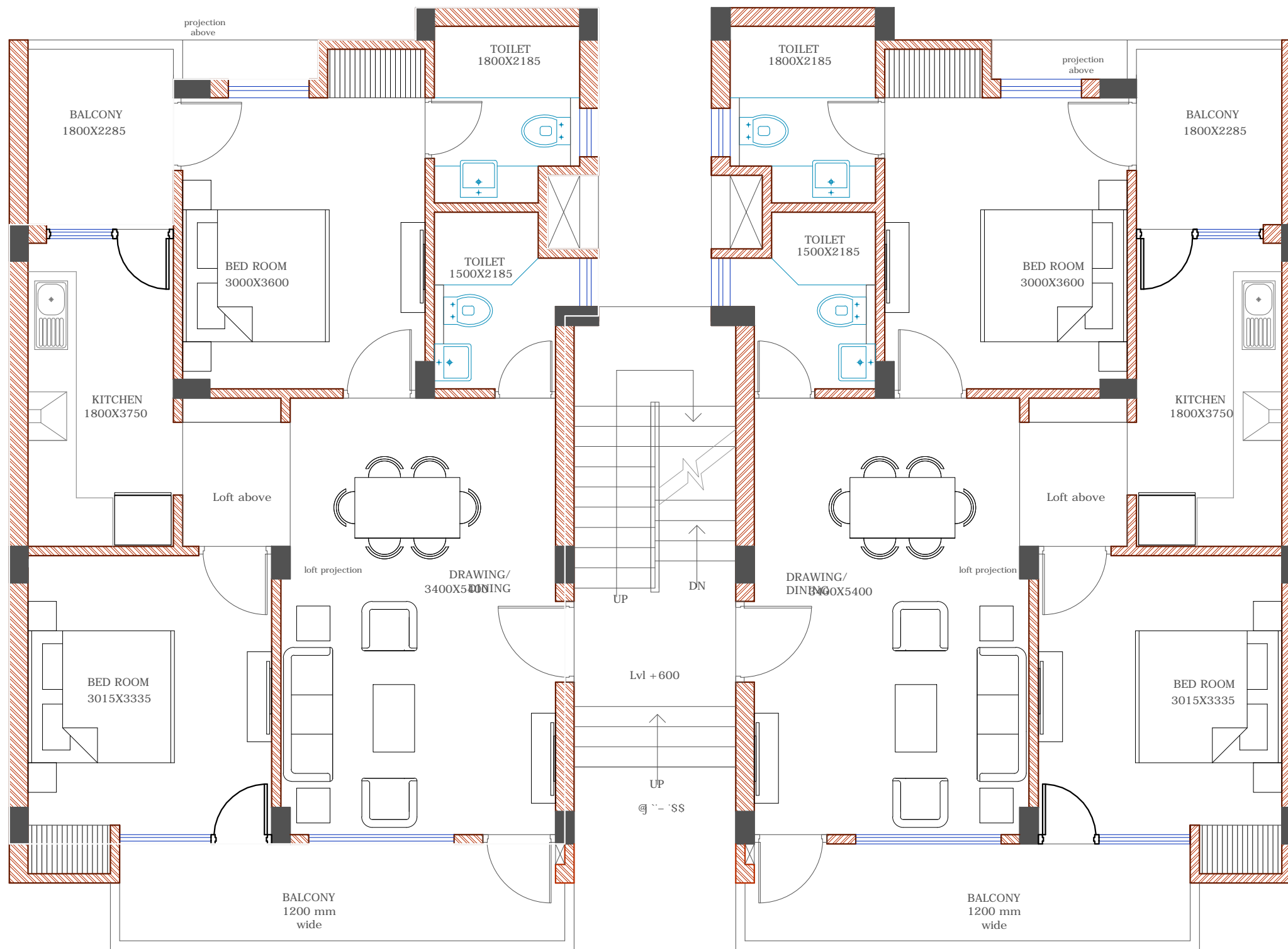
GROUND FLOOR PLAN 2 BED ROOM APARTMENT TYPE- B
